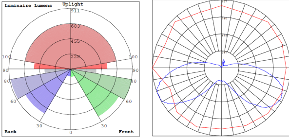
BUG Rating: B2-U4-G3
